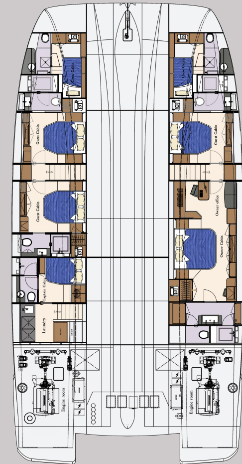
Lower Deck
